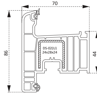
PDR5260BY Dışa Kanat Profili Outside Sash Profile
