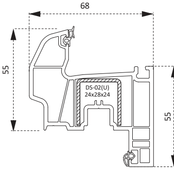
PV70760BY Damlalıklı Kanat Profili Drained Sash Profile
