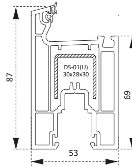
PSY4665BY Fix Kasa Profili Fix Frame Profile
