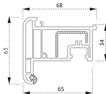
Stump Profile Stump Profile PR7113
