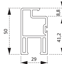
PSY4865BY Sineklikli Kanat Profili Sash Fly Screen Profile
