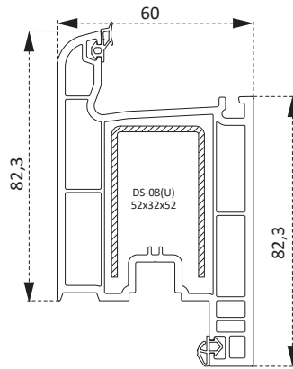
PVN0460BY Kapı Profili Opening Door Profile
