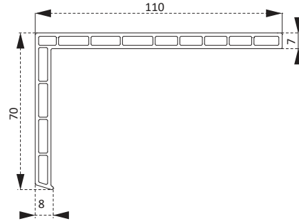
PTS3560BY Pervaz Profili Casing Profile
