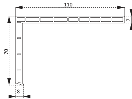
PTS3560BY Pervaz Profili Casing Profile
