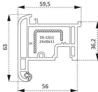
PVN1360BY Stump Profili Stump Profile
