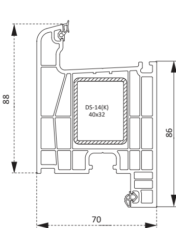
PDR0460BY Kapı Profili Opening Door Profile
