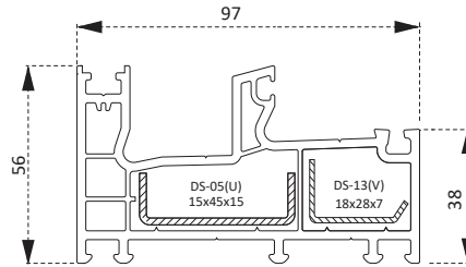
PSY4665BY Fix Kasa Profili Fix Frame Profile
