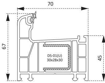
PDR0160BY Kasa Profili Frame Profile
