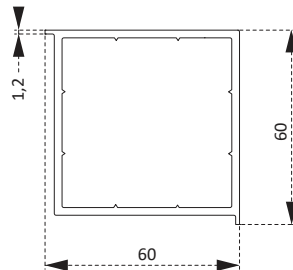
PEX3360BY Kutu Profili Box Profile
