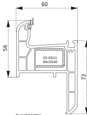
PVN0860BY Pervazlı Kasa Profili Casing Frame Profile
