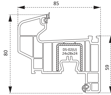
PDR0760BY Damlalıklı Kanat Profili Drained Sash Profile
