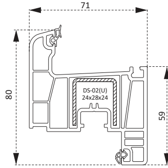
PDR0260BY Kanat Profili Sash Profile
