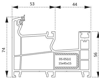
PSY5165BY Dış Fix Kasa Profili Outside Fix Frame Profile
