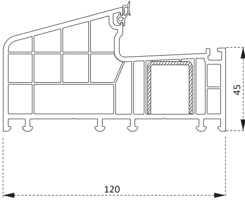
PRHL01 Kasa Profili Frame Profile
