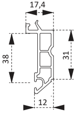
PTS3660BY Dekoratif Pervaz Profili Decorative Casing Profile
