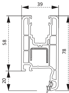
PS60260BY Kanat Profili Sash Profile
