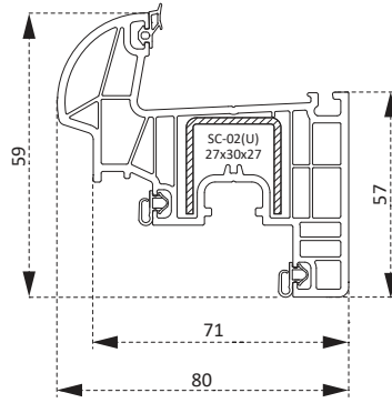
PSC0260BY Damlalıklı Kanat Profili Drained Sash Profile
