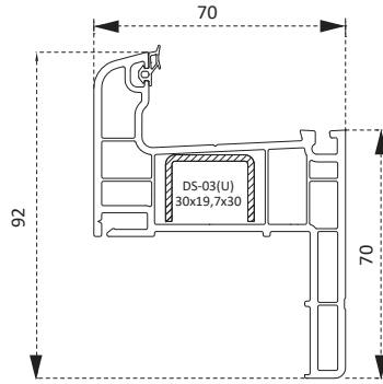
PDR0860BY Pervazlı Kasa Profili Casing Frame Profile
