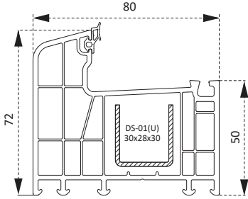
PGR0160BY Kasa Profili Frame Profile
