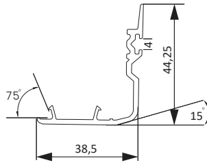
PRS638 Kanat Adaptörü Sliding Sash Adapter
