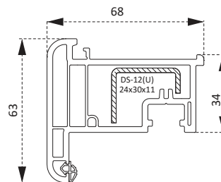
PDR1360BY Stümp Profili Stump Profile
