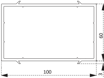
PEX3460BY Kutu Profili Box Profile
