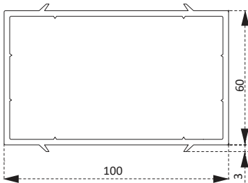
PEX3460BY Kutu Profili Box Profile
