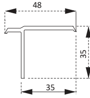
PTS3160BY Asimetrik T T Covering
