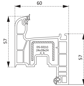
PVN0260BY Kanat Profili Sash Profile
