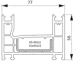
PSY0165BY Kasa Profili Frame Profile
