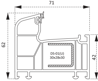
PV70160BY Kasa Profili Frame Profile
