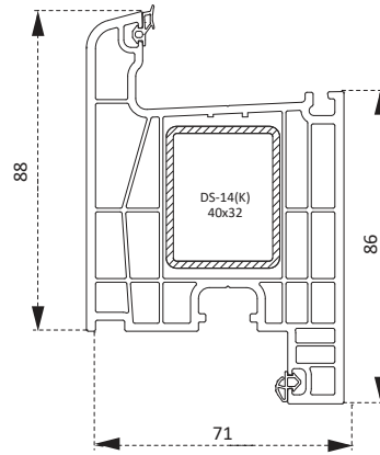
PDR0460BY Kapı Profili Opening Door Profile
