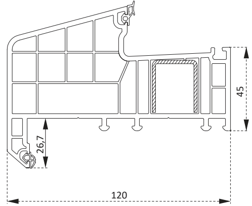
PRHL08 Pervazlı Kasa Profili Casing Frame Profile
