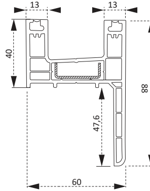
PS60860BY Pervazlı Kasa Profili Casing Frame Profile
