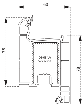
PRVNEC04B Kapı Profili Opening Door Profile
