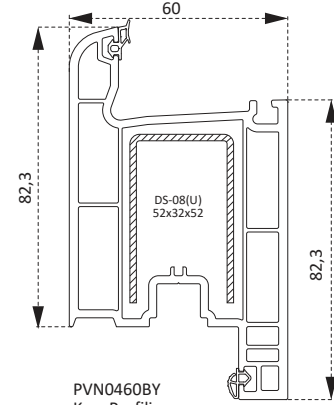
PVN0460BY Kapı Profili Opening Door Profile
