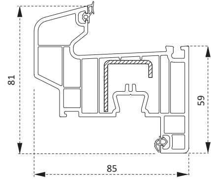
PR7107 Damlalıklı Kanat Profili Drained Sash Profile
