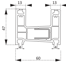
PS60160BY Kasa Profili Frame Profile
